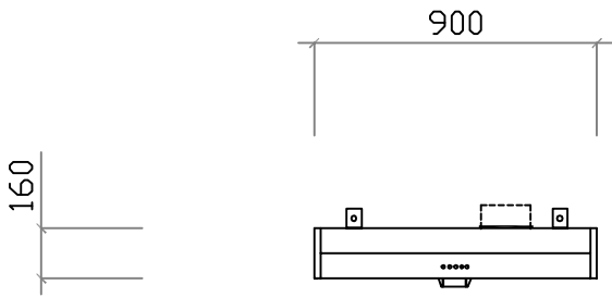
FRONT VIEW (mm)
